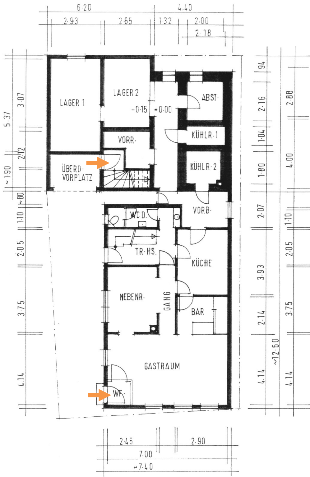
GH.846 – Grundriss EG
