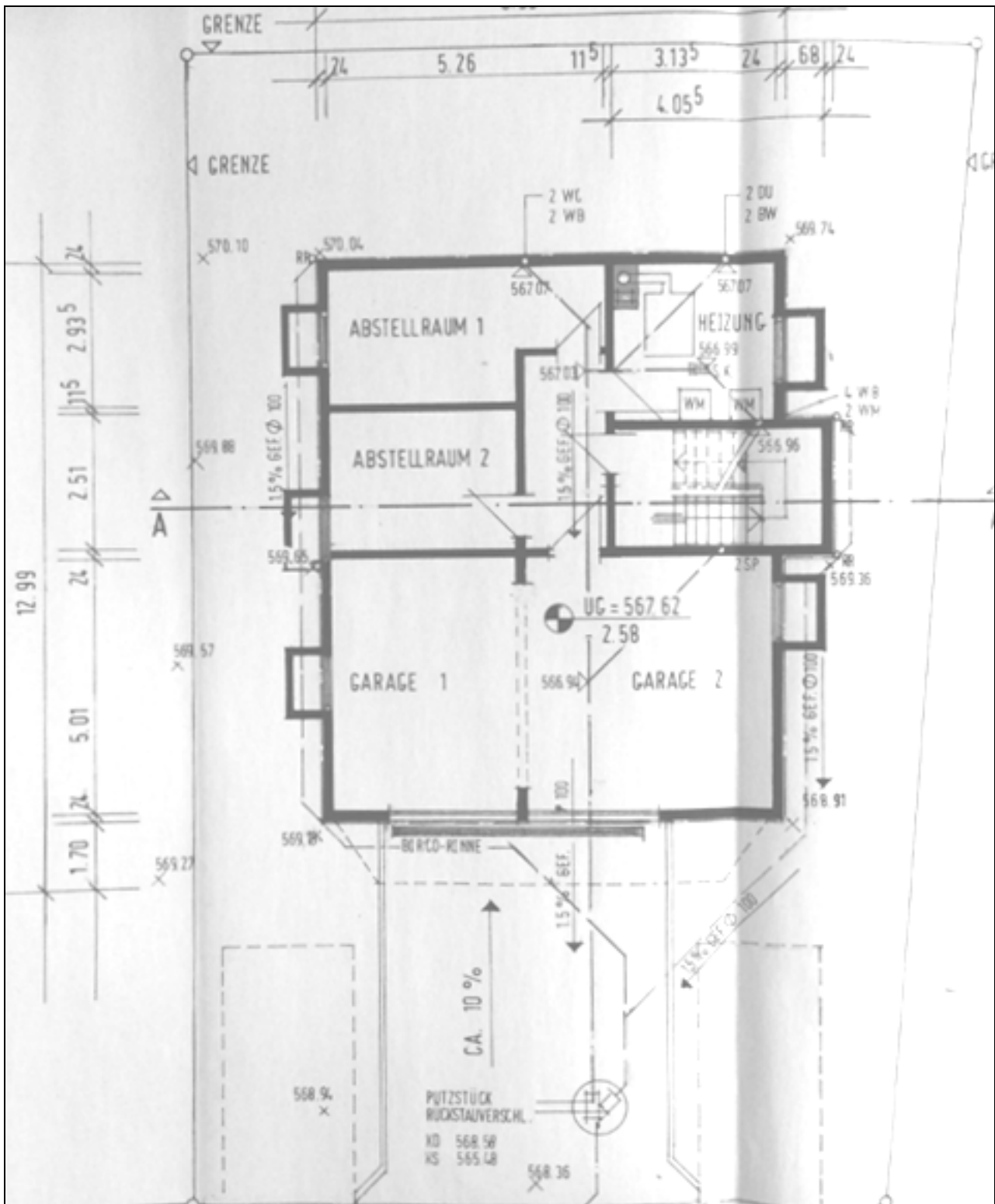
GH.842 – UG Grundriss
