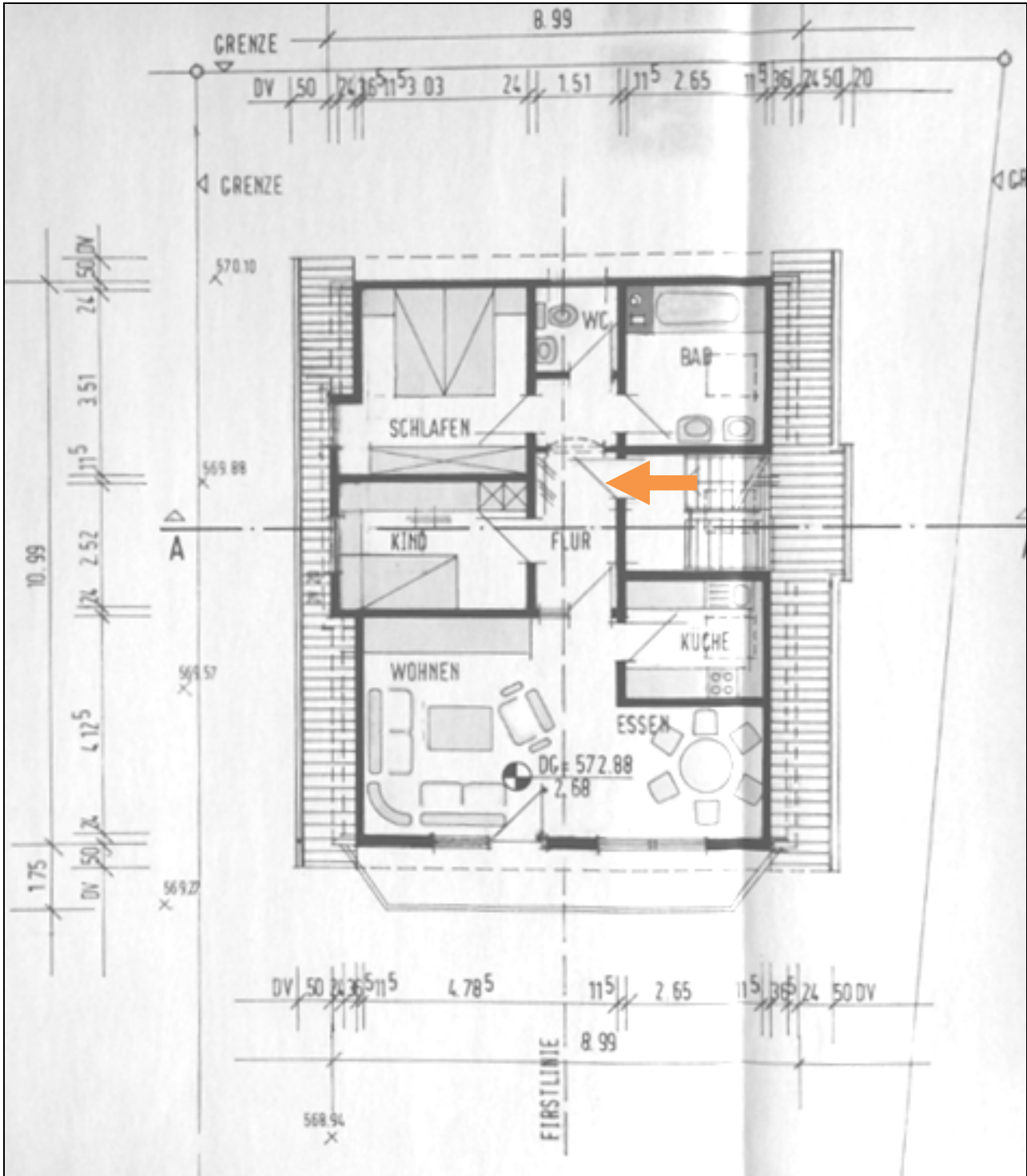
GH.842 – DG Grundriss
