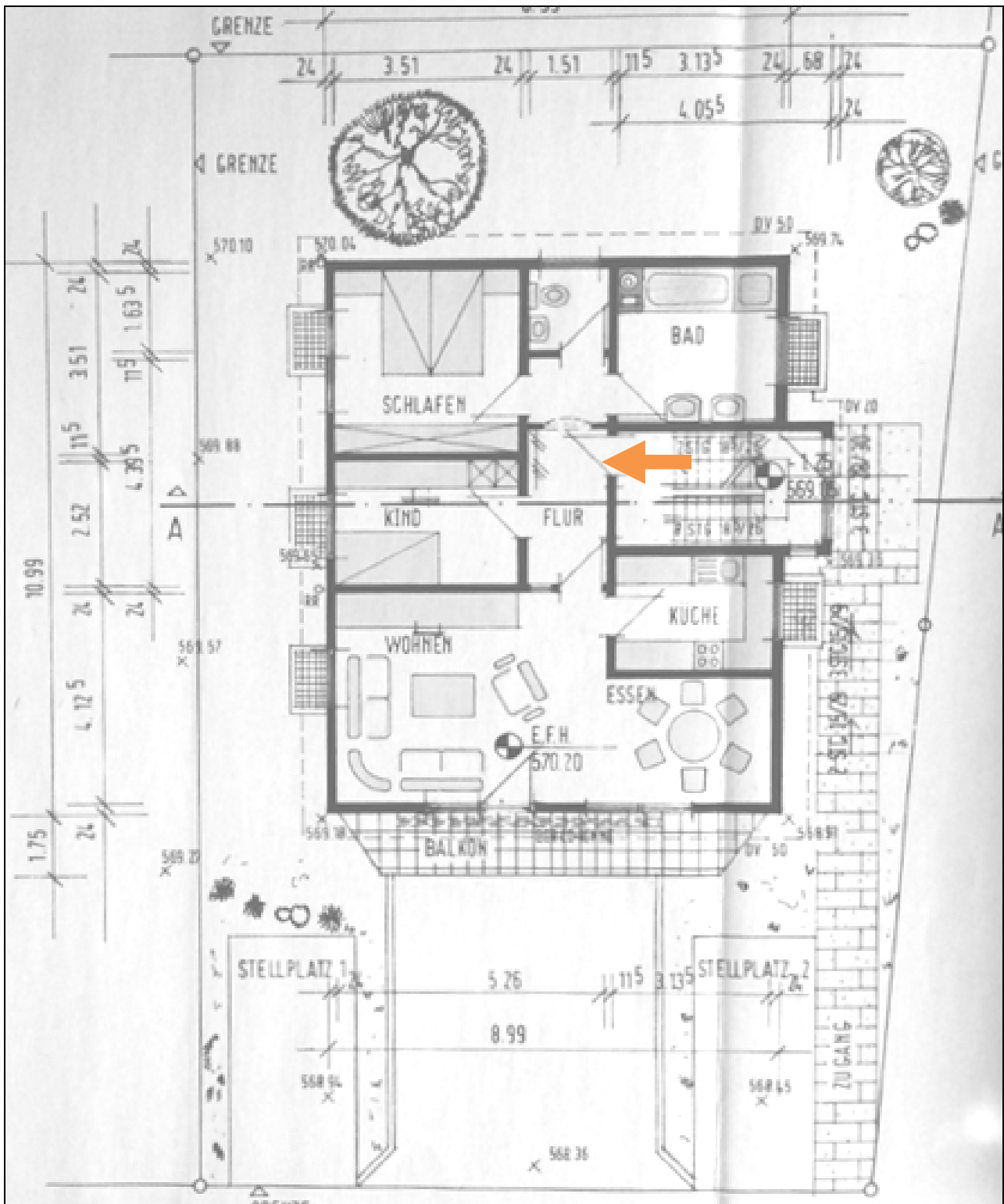
GH.842 – EG Grundriss
